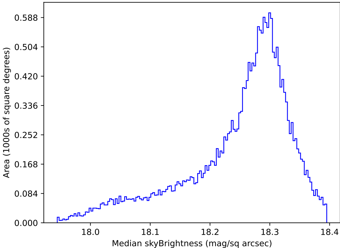
ddf_loaded_fl4_v3.4_10yrs All sky y band: Median skyBrightness
