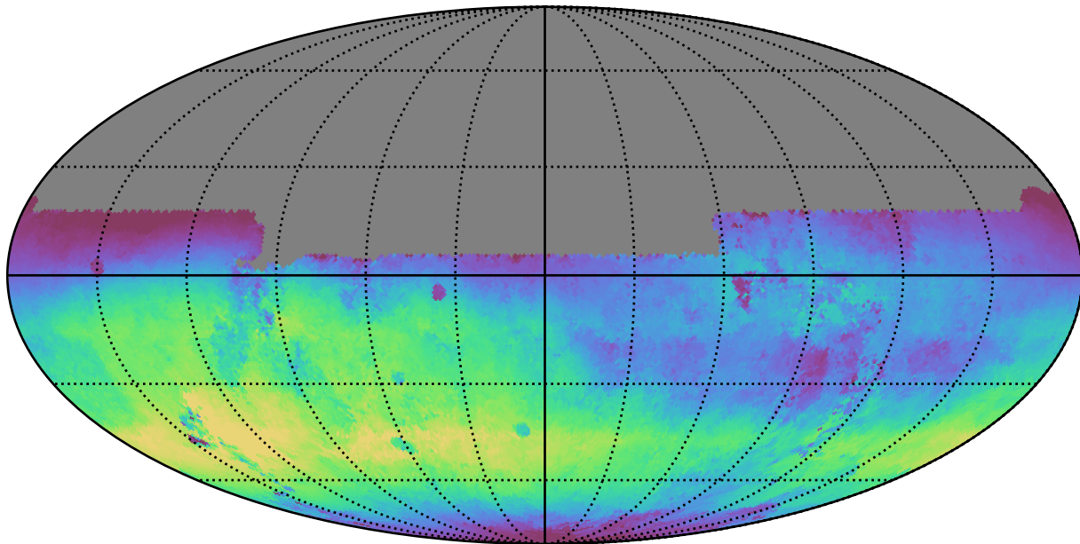
ddf_loaded_fl4_v3.4_10yrs All sky u band: Median skyBrightness
