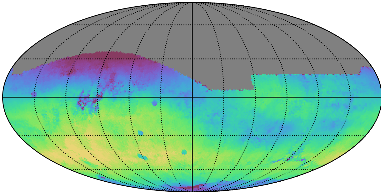
ddf_loaded_fl4_v3.4_10yrs All sky r band: Median skyBrightness
