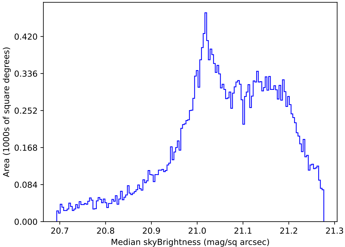
ddf_loaded_fl4_v3.4_10yrs All sky r band: Median skyBrightness
