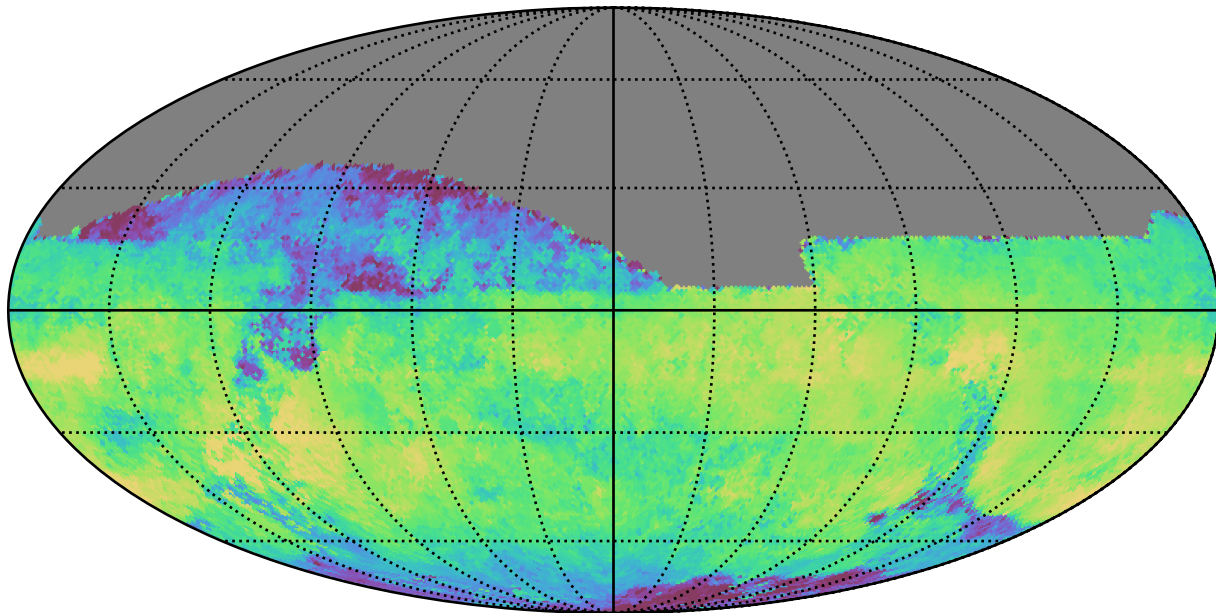
ddf_loaded_fl4_v3.4_10yrs All sky i band: Median skyBrightness
