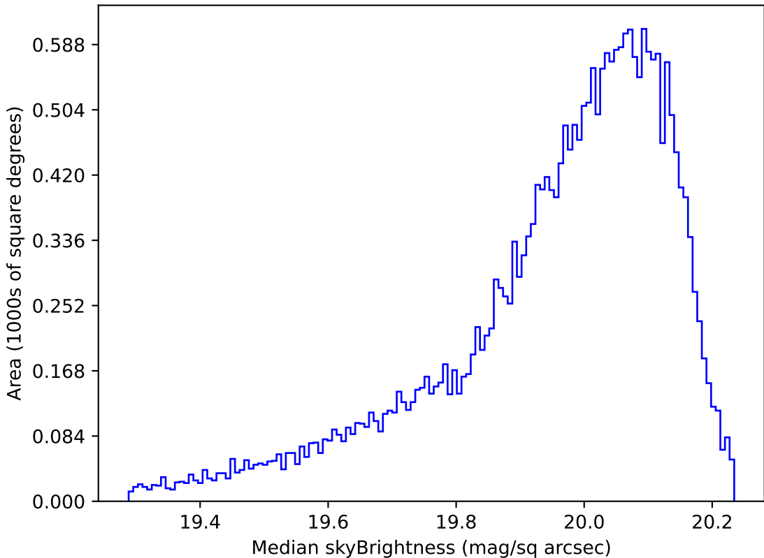
ddf_loaded_fl4_v3.4_10yrs All sky i band: Median skyBrightness
