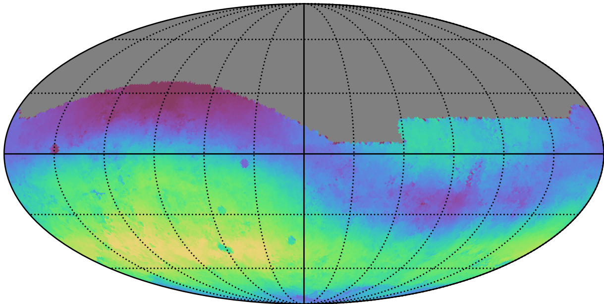
ddf_loaded_fl4_v3.4_10yrs All sky g band: Median skyBrightness
