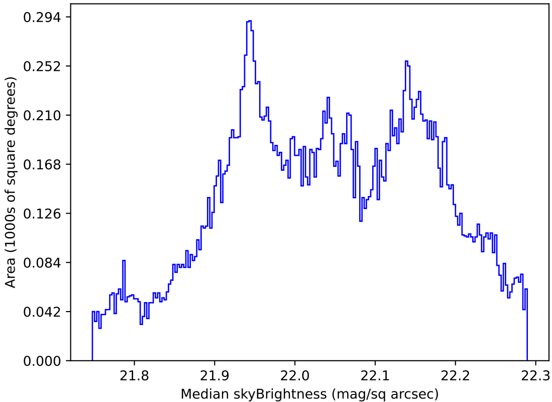
ddf_loaded_fl4_v3.4_10yrs All sky g band: Median skyBrightness
