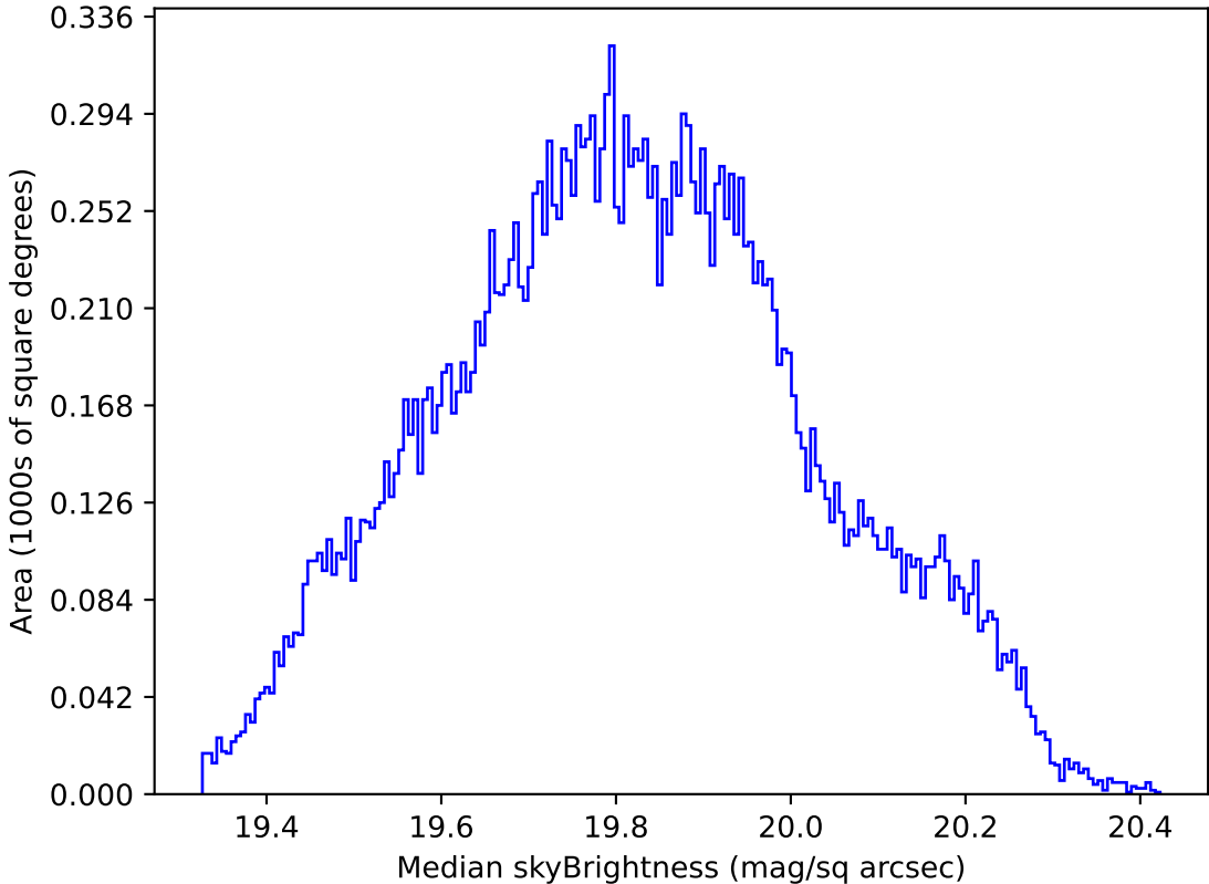
ddf_loaded_fl4_v3.4_10yrs All sky all bands: Median skyBrightness
