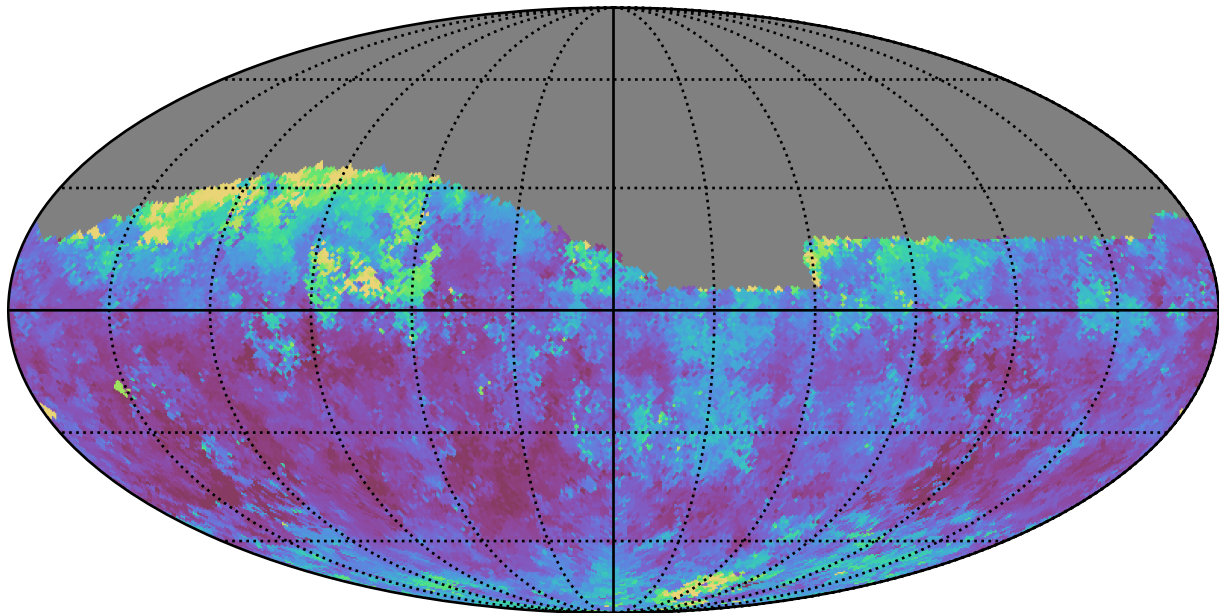
ddf_loaded_fl4_v3.4_10yrs Yr 1 z band: Median seeingGeom
