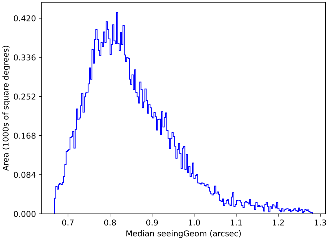
ddf_loaded_fl4_v3.4_10yrs Yr 1 z band: Median seeingGeom
