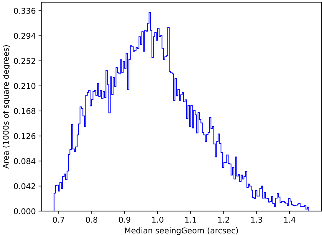
ddf_loaded_fl4_v3.4_10yrs Yr 1 u band: Median seeingGeom
