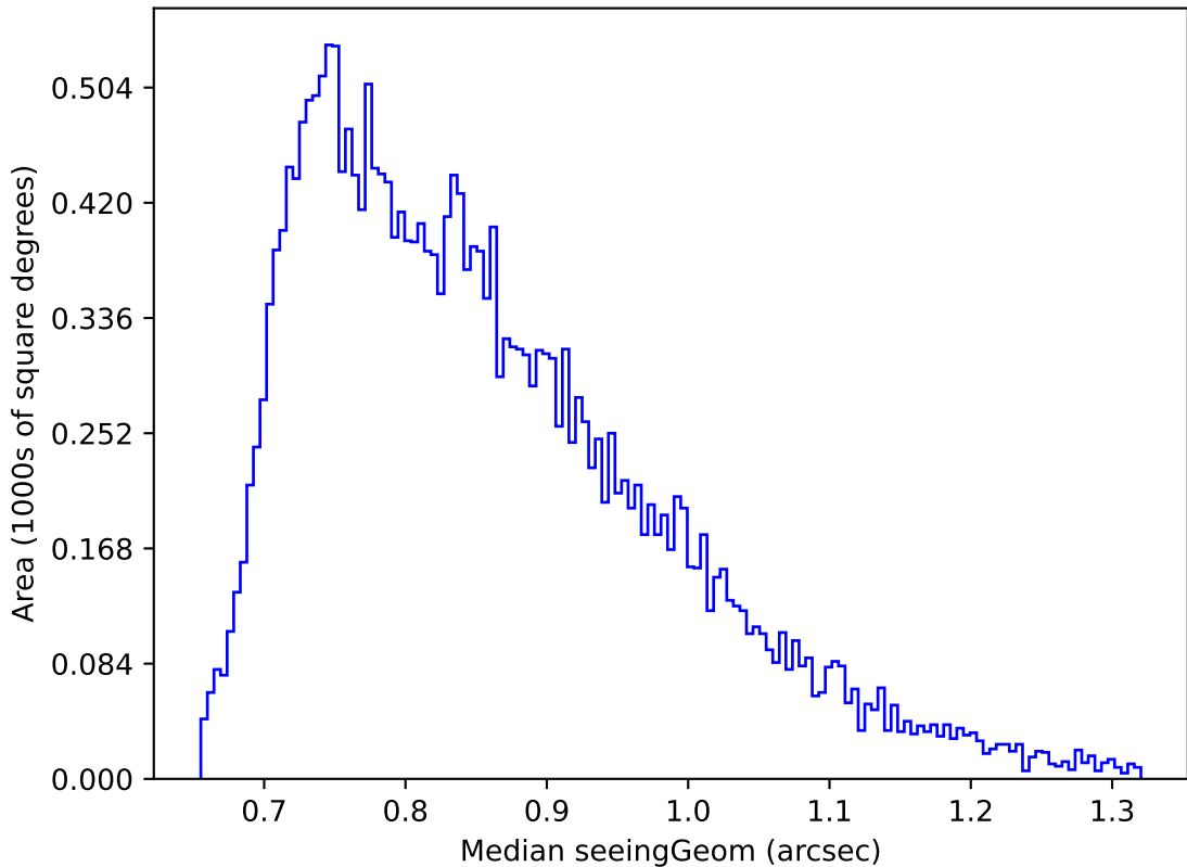
ddf_loaded_fl4_v3.4_10yrs Yr 1 r band: Median seeingGeom
