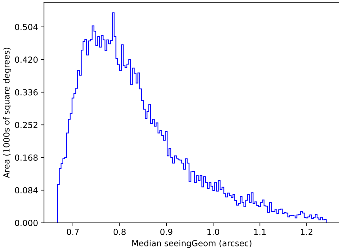
ddf_loaded_fl4_v3.4_10yrs Yr 1 i band: Median seeingGeom
