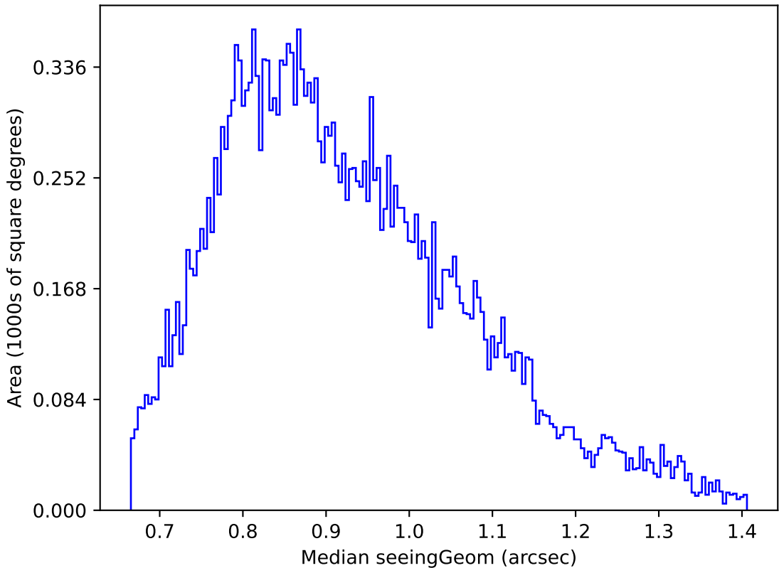
ddf_loaded_fl4_v3.4_10yrs Yr 1 g band: Median seeingGeom
