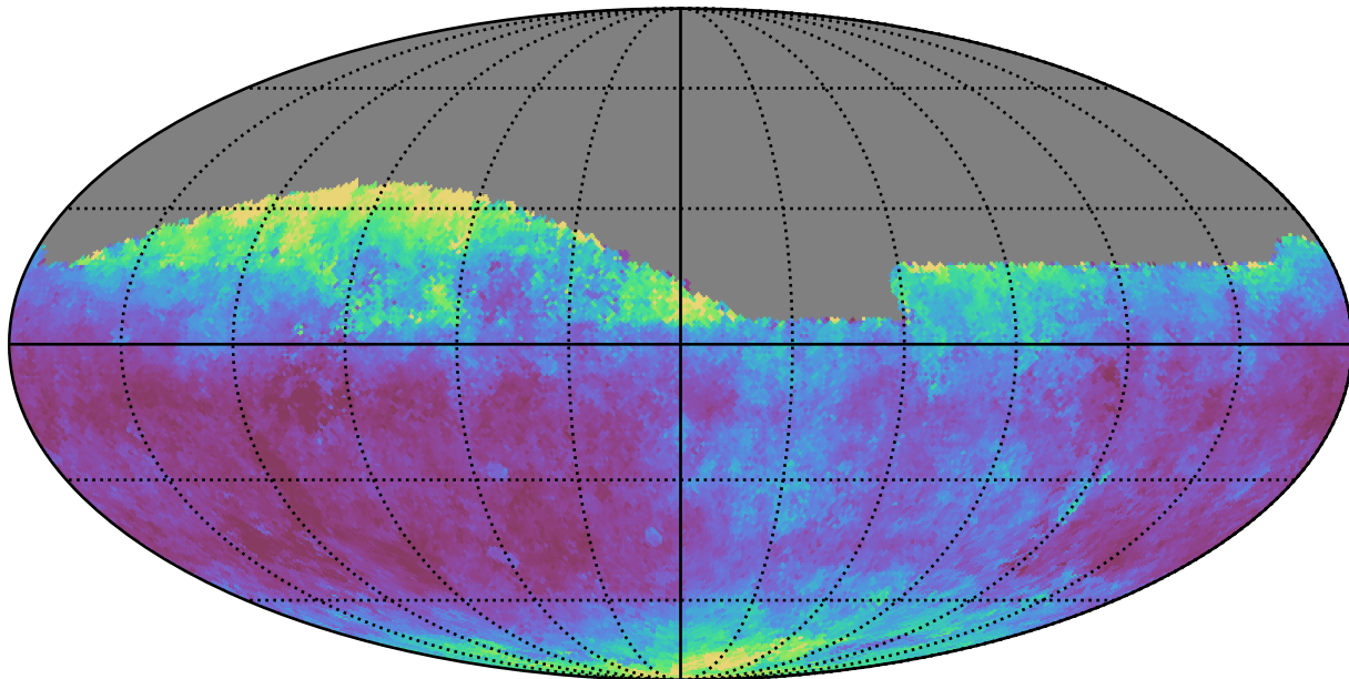
ddf_loaded_fl4_v3.4_10yrs Yr 1 all bands: Median seeingGeom
