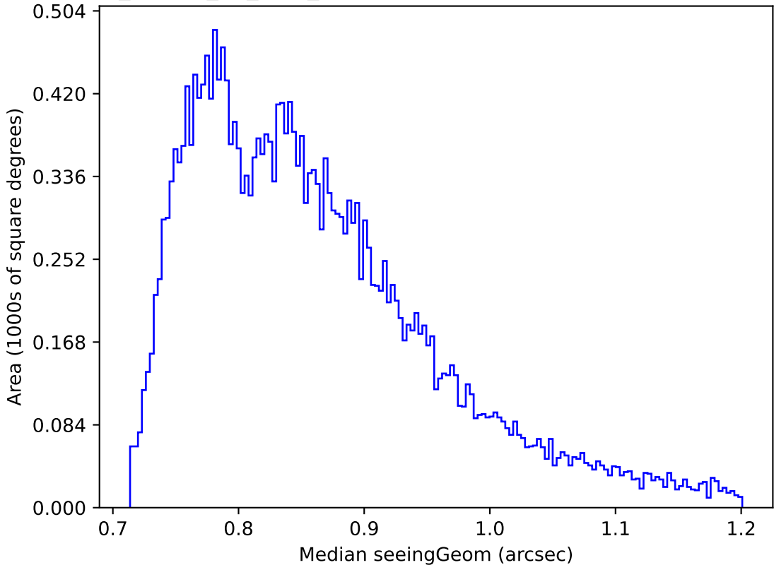
ddf_loaded_fl4_v3.4_10yrs Yr 1 all bands: Median seeingGeom
