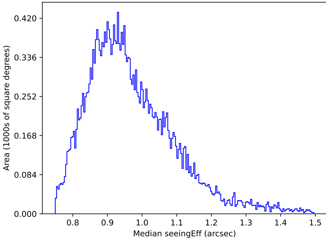
ddf_loaded_fl4_v3.4_10yrs Yr 1 z band: Median seeingEff
