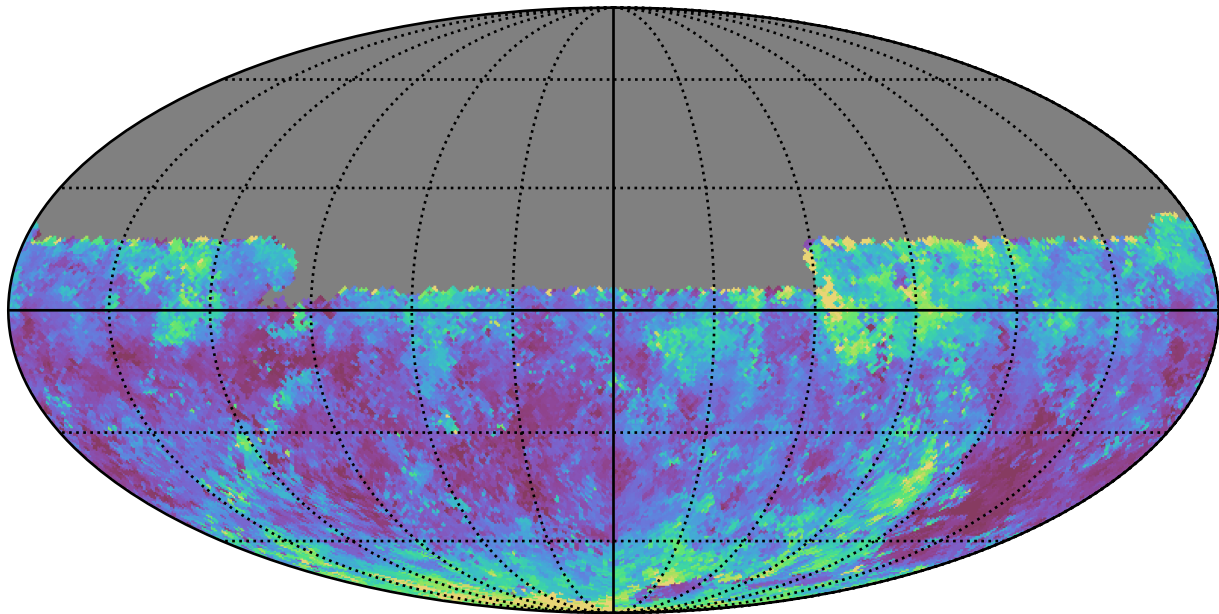
ddf_loaded_fl4_v3.4_10yrs Yr 1 y band: Median seeingEff
