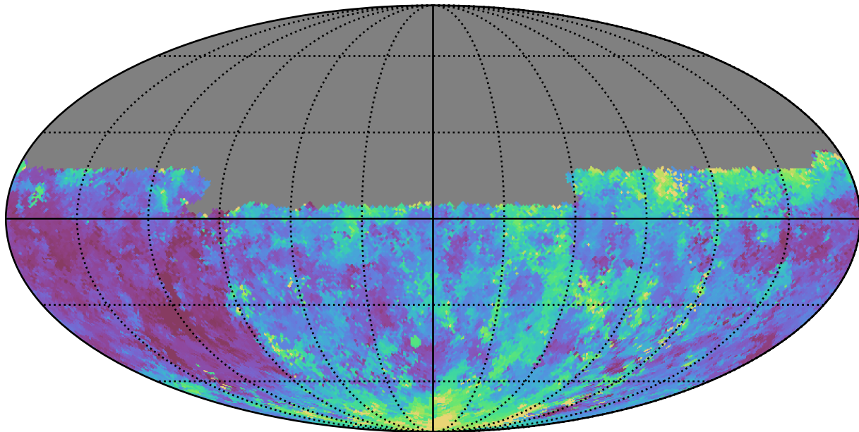
ddf_loaded_fl4_v3.4_10yrs Yr 1 u band: Median seeingEff
