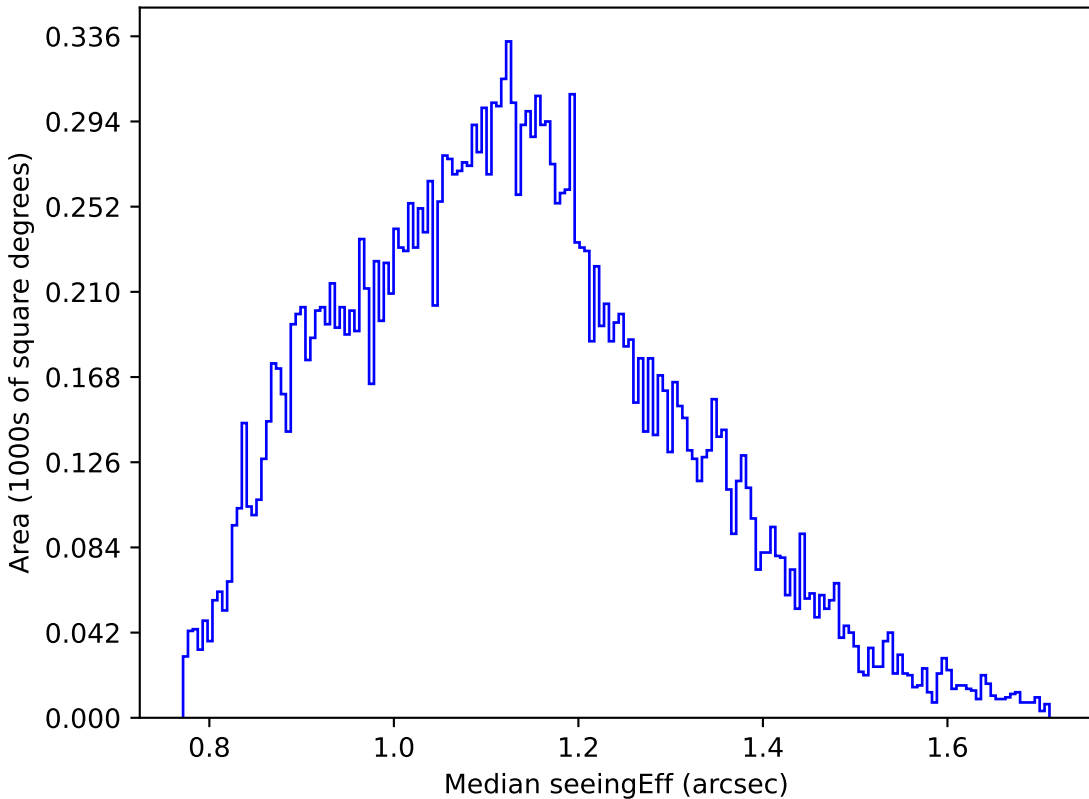
ddf_loaded_fl4_v3.4_10yrs Yr 1 u band: Median seeingEff
