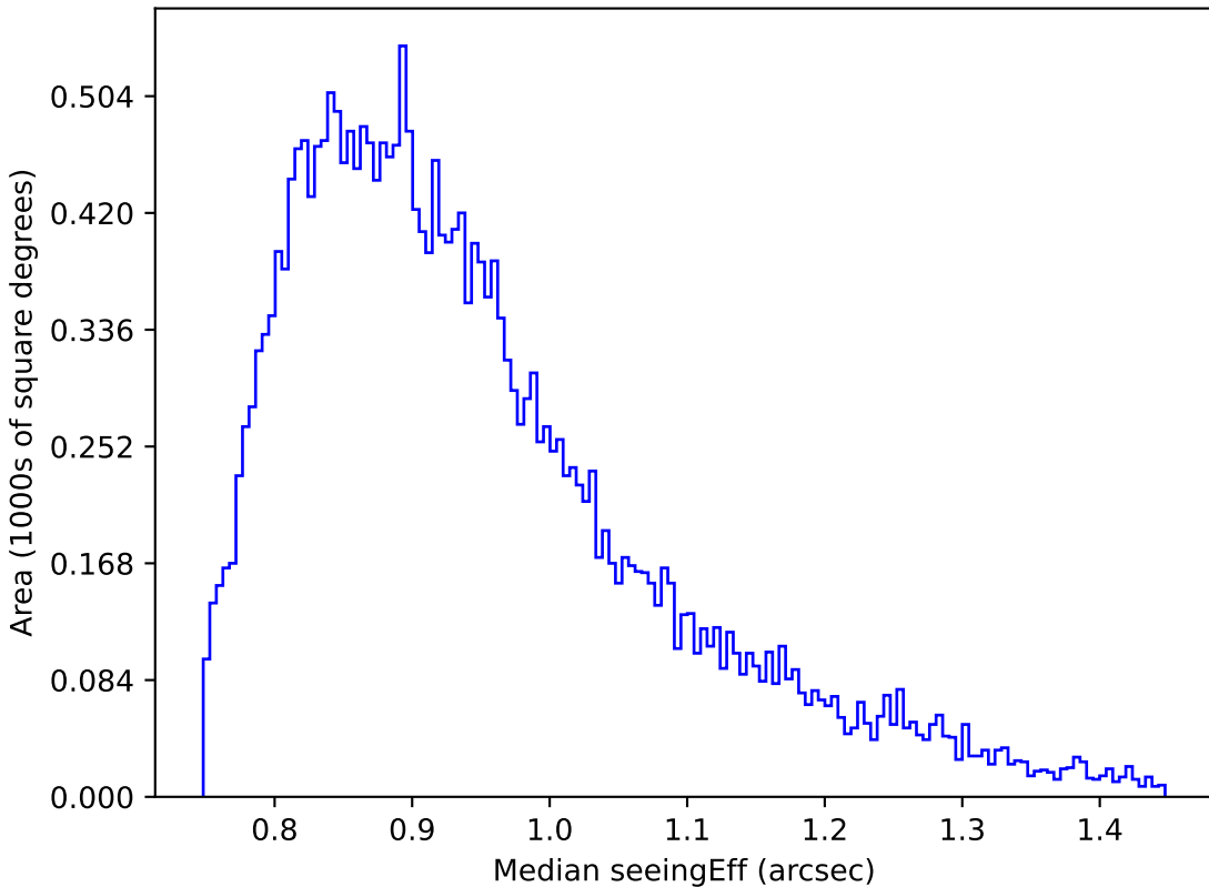
ddf_loaded_fl4_v3.4_10yrs Yr 1 i band: Median seeingEff
