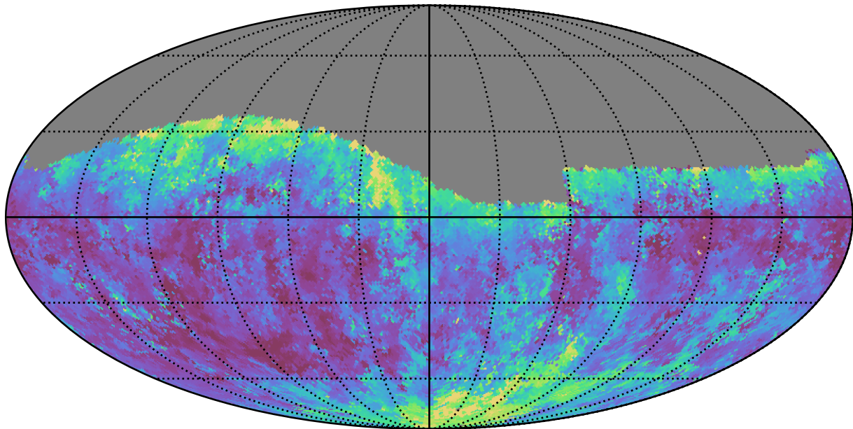
ddf_loaded_fl4_v3.4_10yrs Yr 1 g band: Median seeingEff
