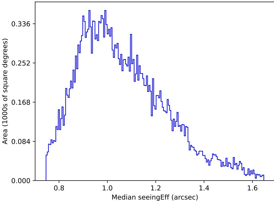
ddf_loaded_fl4_v3.4_10yrs Yr 1 g band: Median seeingEff
