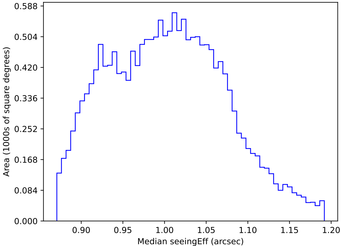
ddf_loaded_fl4_v3.4_10yrs WFD z band: Median seeingEff
