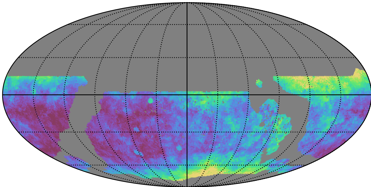
ddf_loaded_fl4_v3.4_10yrs WFD y band: Median seeingEff
