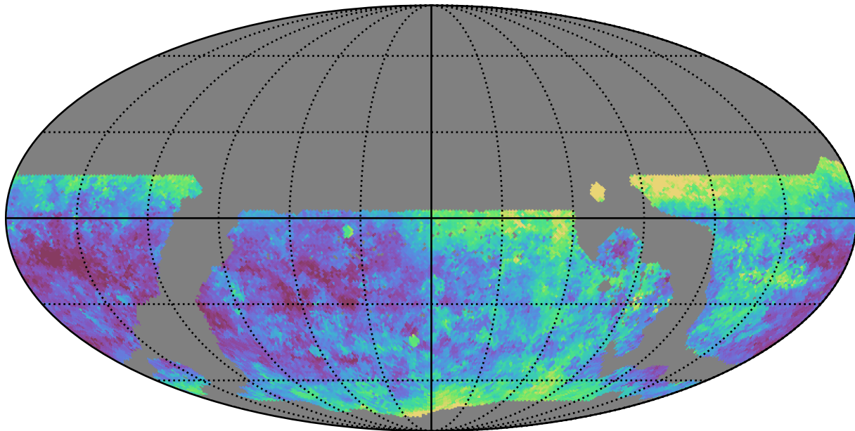
ddf_loaded_fl4_v3.4_10yrs WFD u band: Median seeingEff
