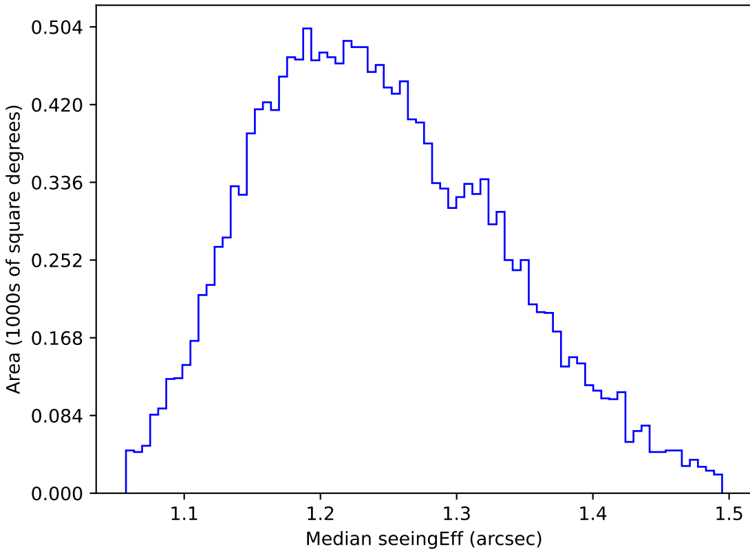
ddf_loaded_fl4_v3.4_10yrs WFD u band: Median seeingEff
