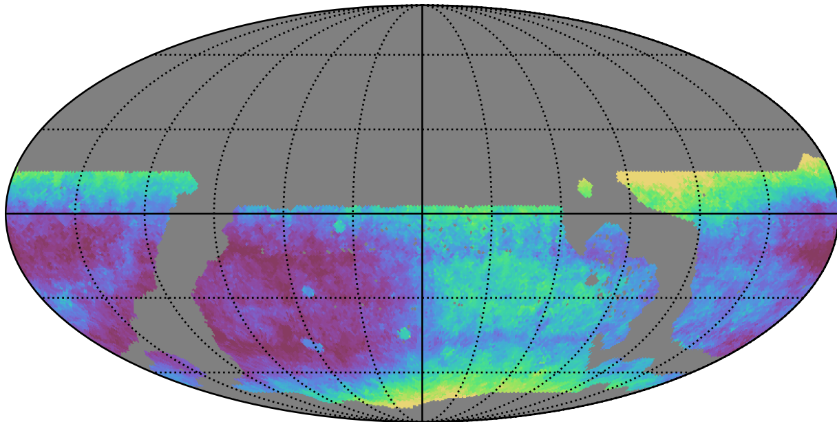
ddf_loaded_fl4_v3.4_10yrs WFD r band: Median seeingEff
