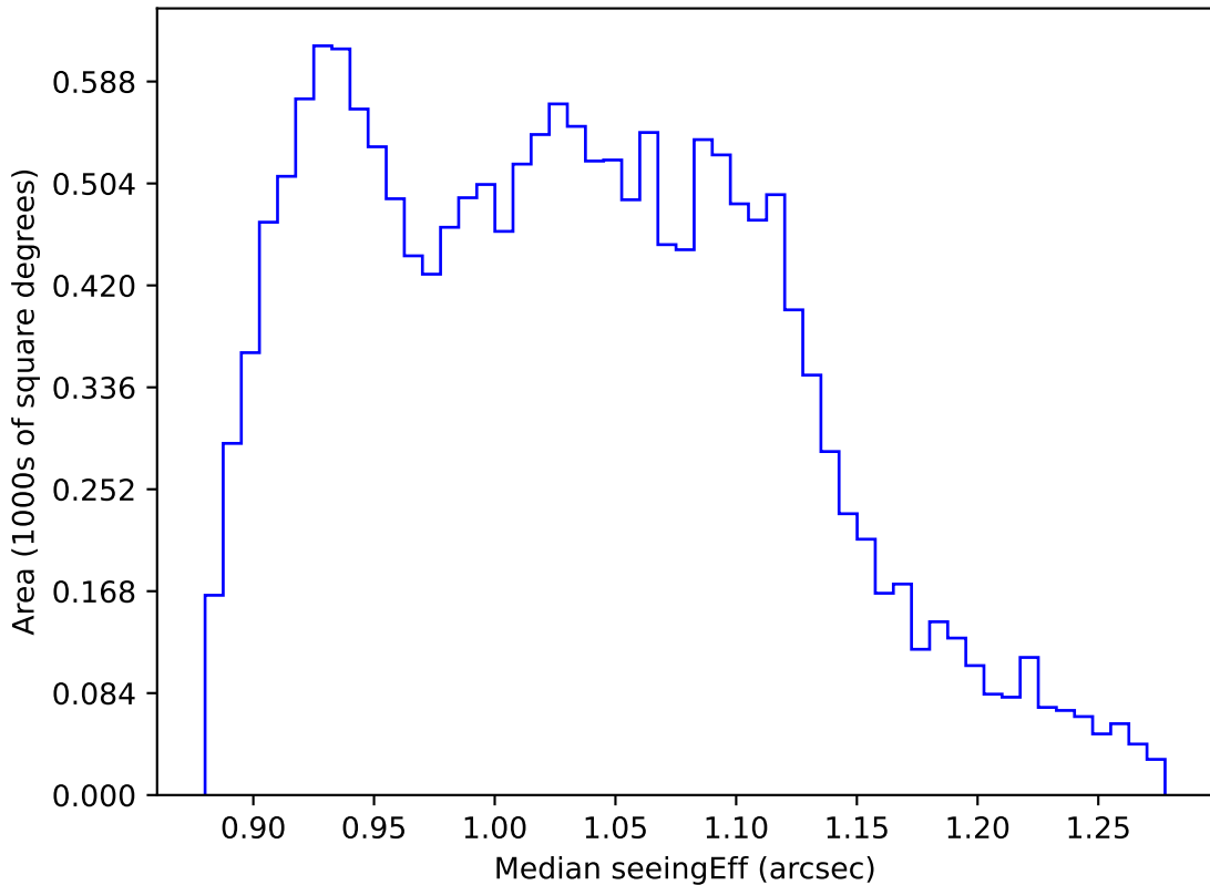
ddf_loaded_fl4_v3.4_10yrs WFD r band: Median seeingEff
