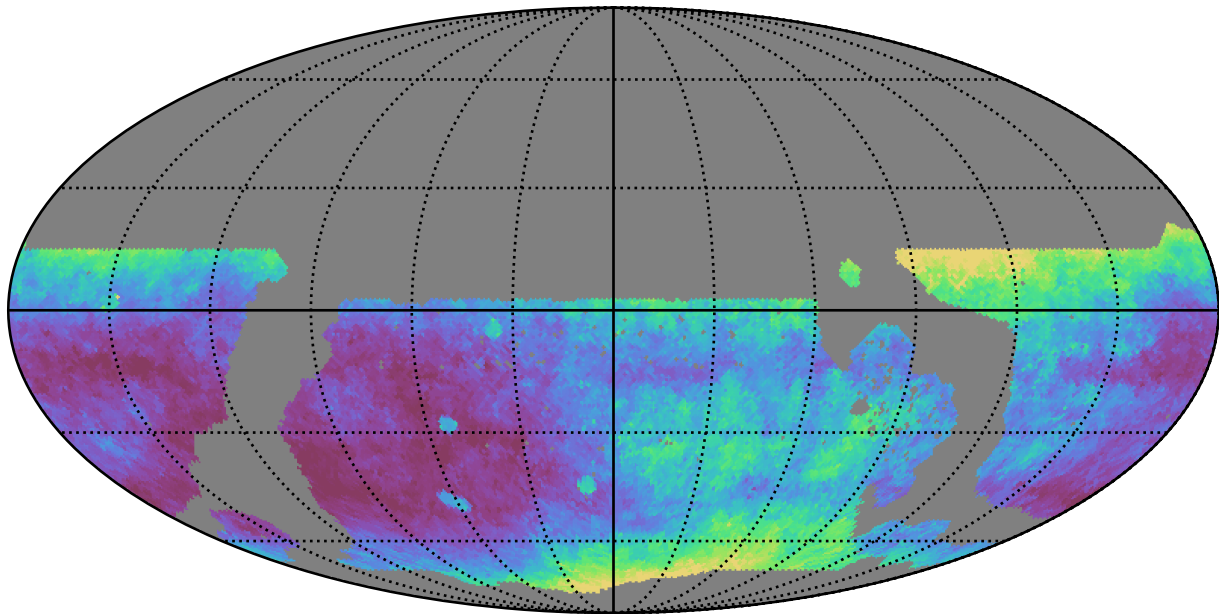
ddf_loaded_fl4_v3.4_10yrs WFD i band: Median seeingEff
