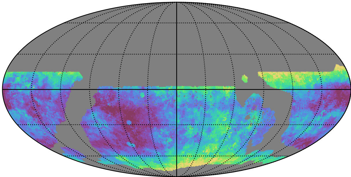
ddf_loaded_fl4_v3.4_10yrs WFD g band: Median seeingEff
