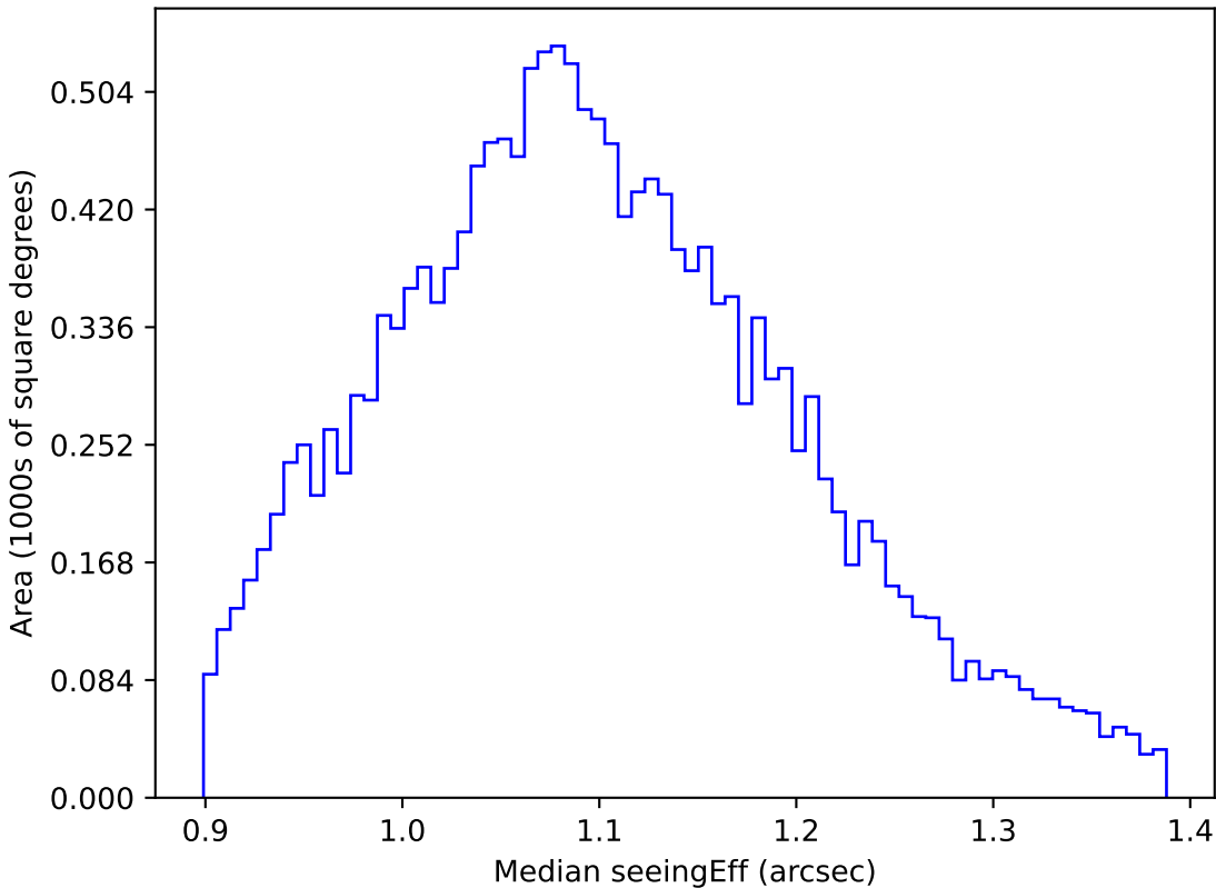
ddf_loaded_fl4_v3.4_10yrs WFD g band: Median seeingEff
