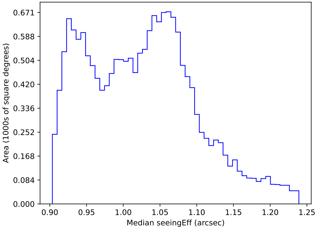
ddf_loaded_fl4_v3.4_10yrs WFD all bands: Median seeingEff
