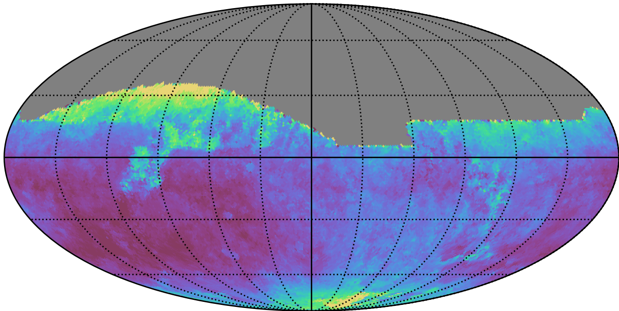
ddf_loaded_fl4_v3.4_10yrs All sky z band: Median seeingEff
