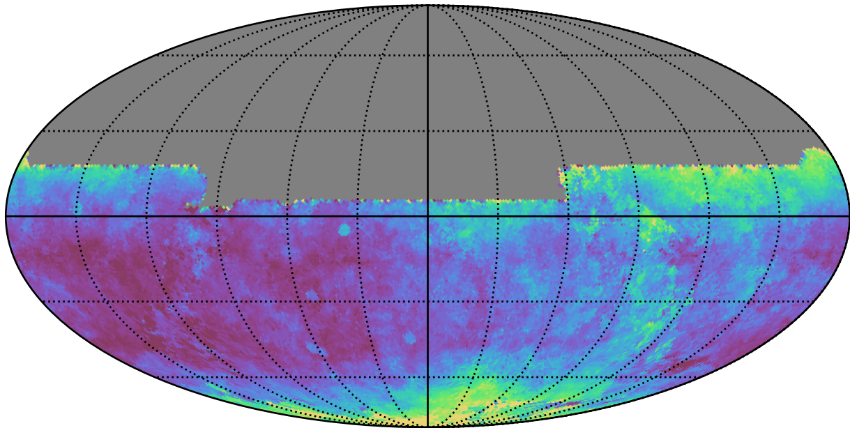
ddf_loaded_fl4_v3.4_10yrs All sky y band: Median seeingEff
