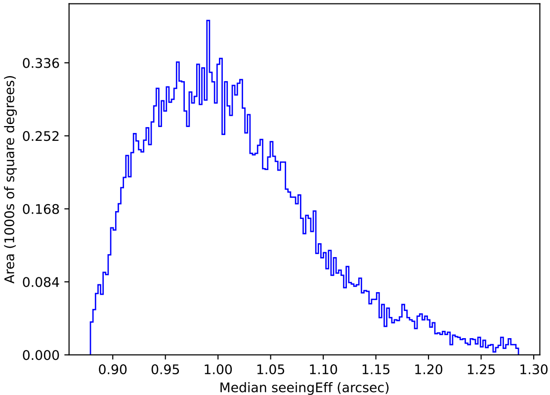
ddf_loaded_fl4_v3.4_10yrs All sky y band: Median seeingEff
