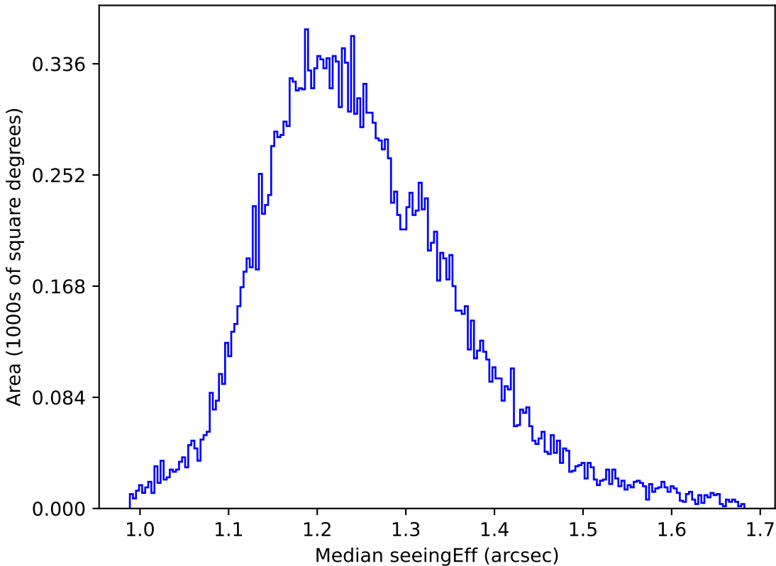
ddf_loaded_fl4_v3.4_10yrs All sky u band: Median seeingEff
