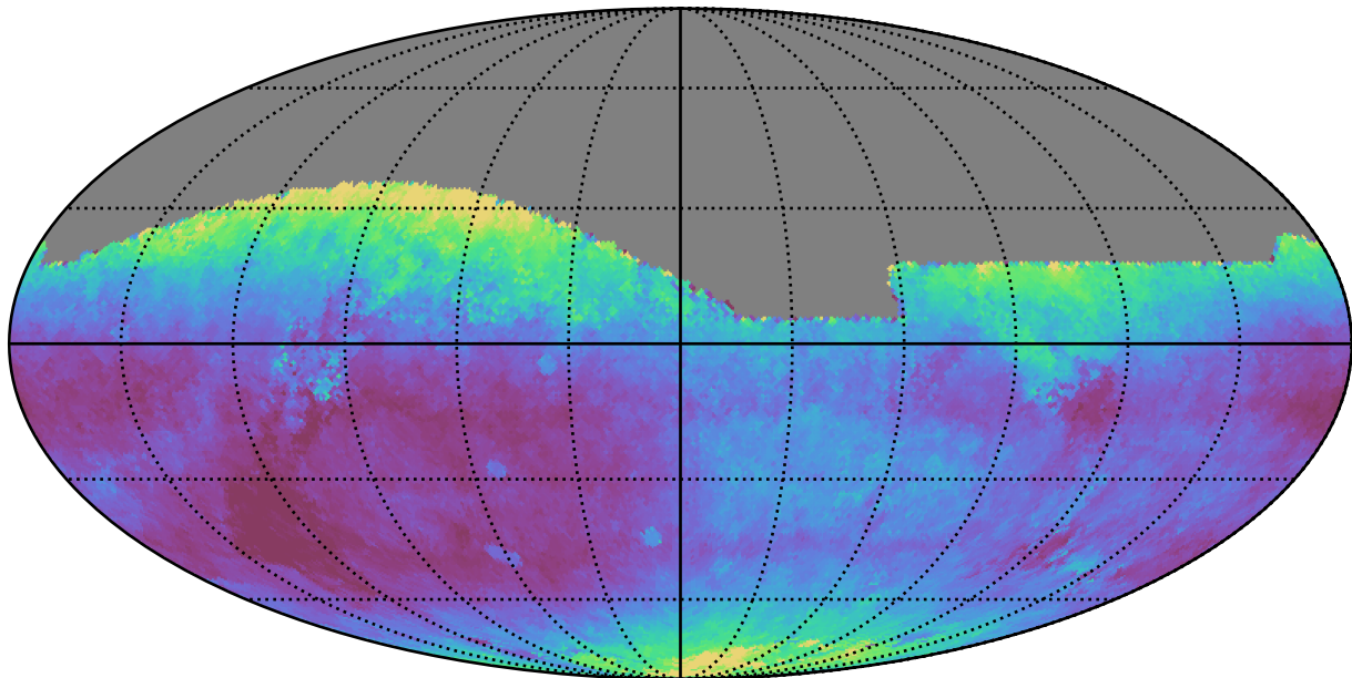
ddf_loaded_fl4_v3.4_10yrs All sky r band: Median seeingEff
