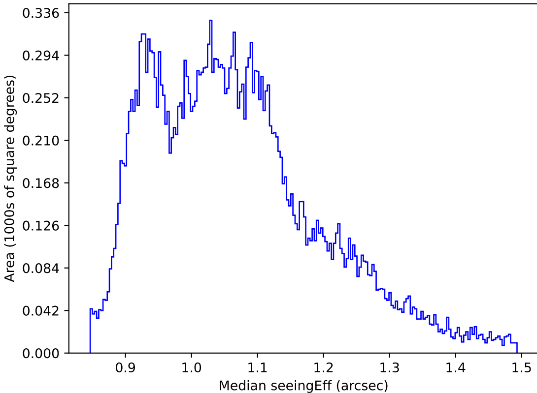
ddf_loaded_fl4_v3.4_10yrs All sky r band: Median seeingEff
