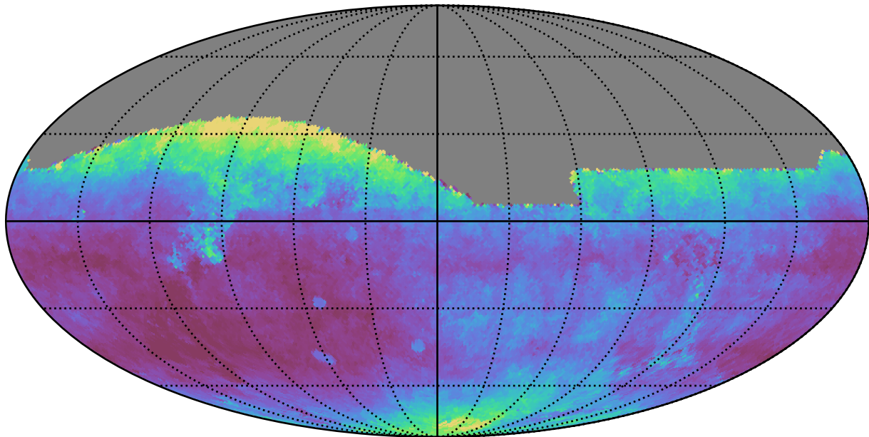
ddf_loaded_fl4_v3.4_10yrs All sky i band: Median seeingEff
