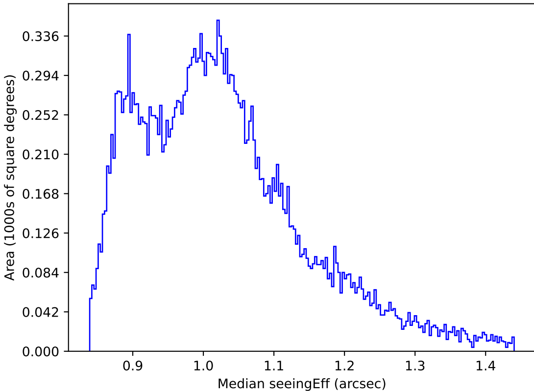
ddf_loaded_fl4_v3.4_10yrs All sky i band: Median seeingEff
