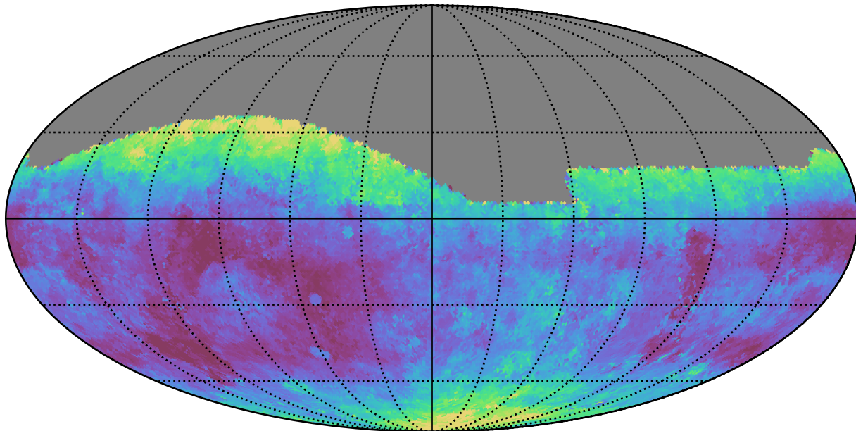
ddf_loaded_fl4_v3.4_10yrs All sky g band: Median seeingEff
