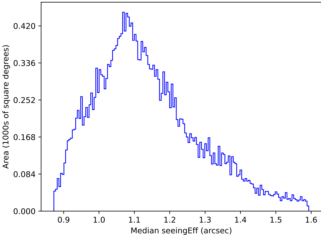
ddf_loaded_fl4_v3.4_10yrs All sky g band: Median seeingEff
