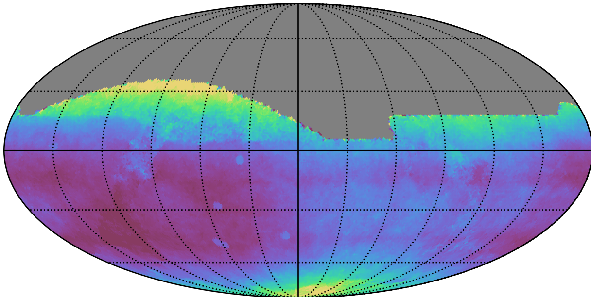
ddf_loaded_fl4_v3.4_10yrs All sky all bands: Median seeingEff
