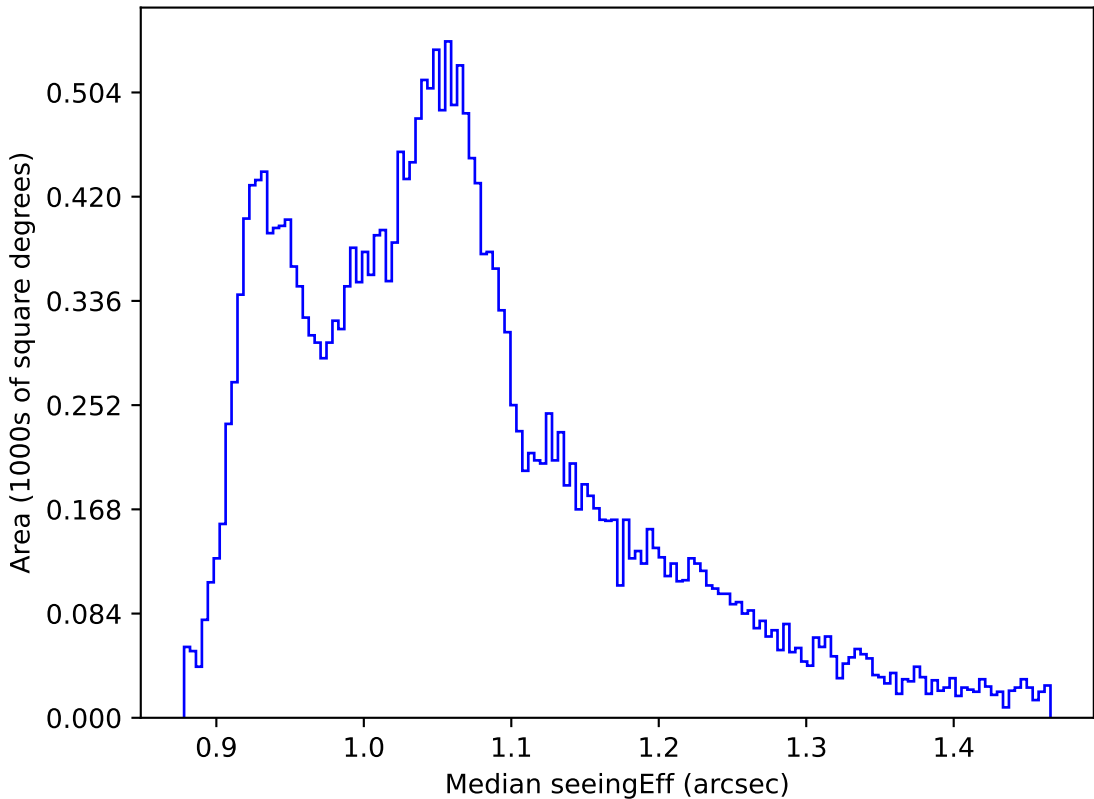
ddf_loaded_fl4_v3.4_10yrs All sky all bands: Median seeingEff
