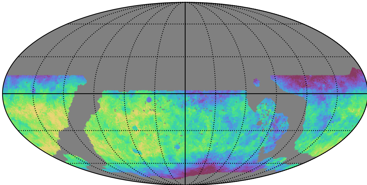
ddf_loaded_fl4_v3.4_10yrs WFD y band: Median saturation_mag
