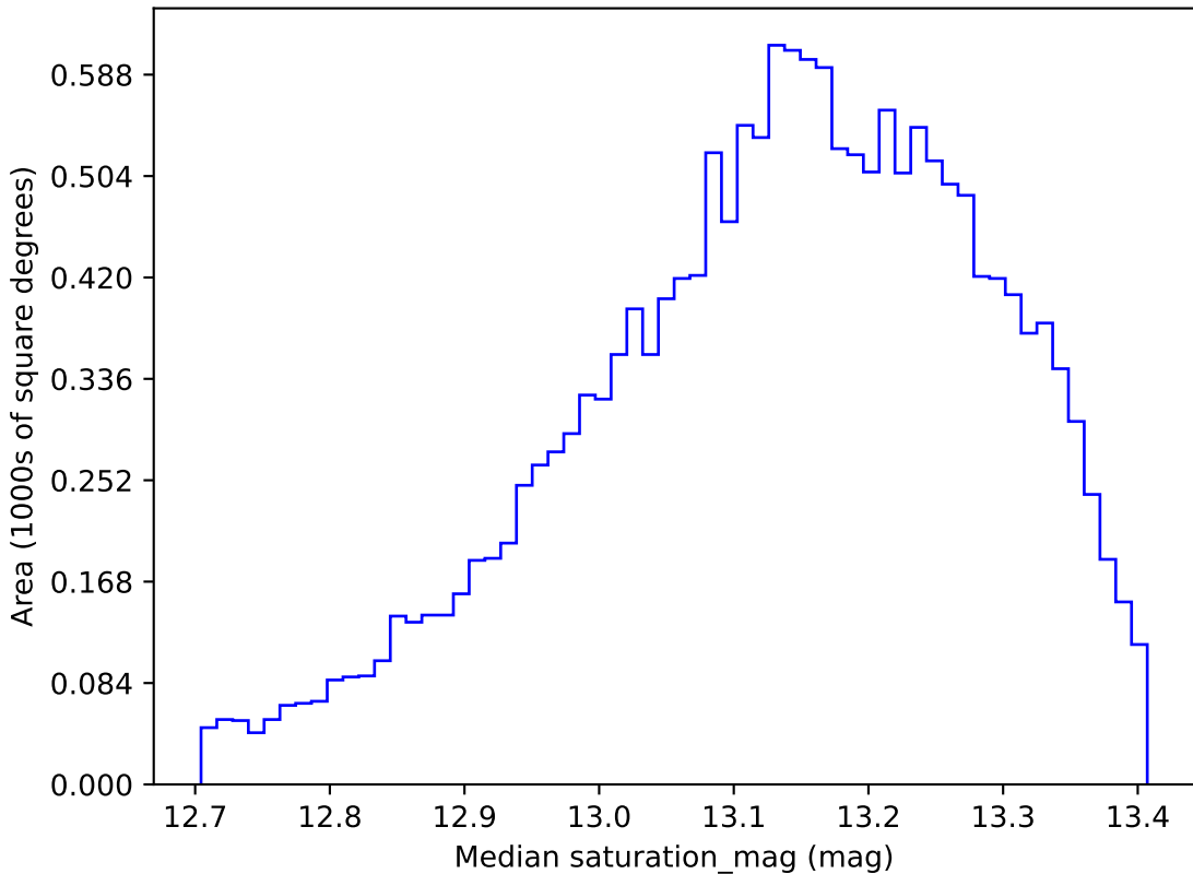
ddf_loaded_fl4_v3.4_10yrs WFD y band: Median saturation_mag
