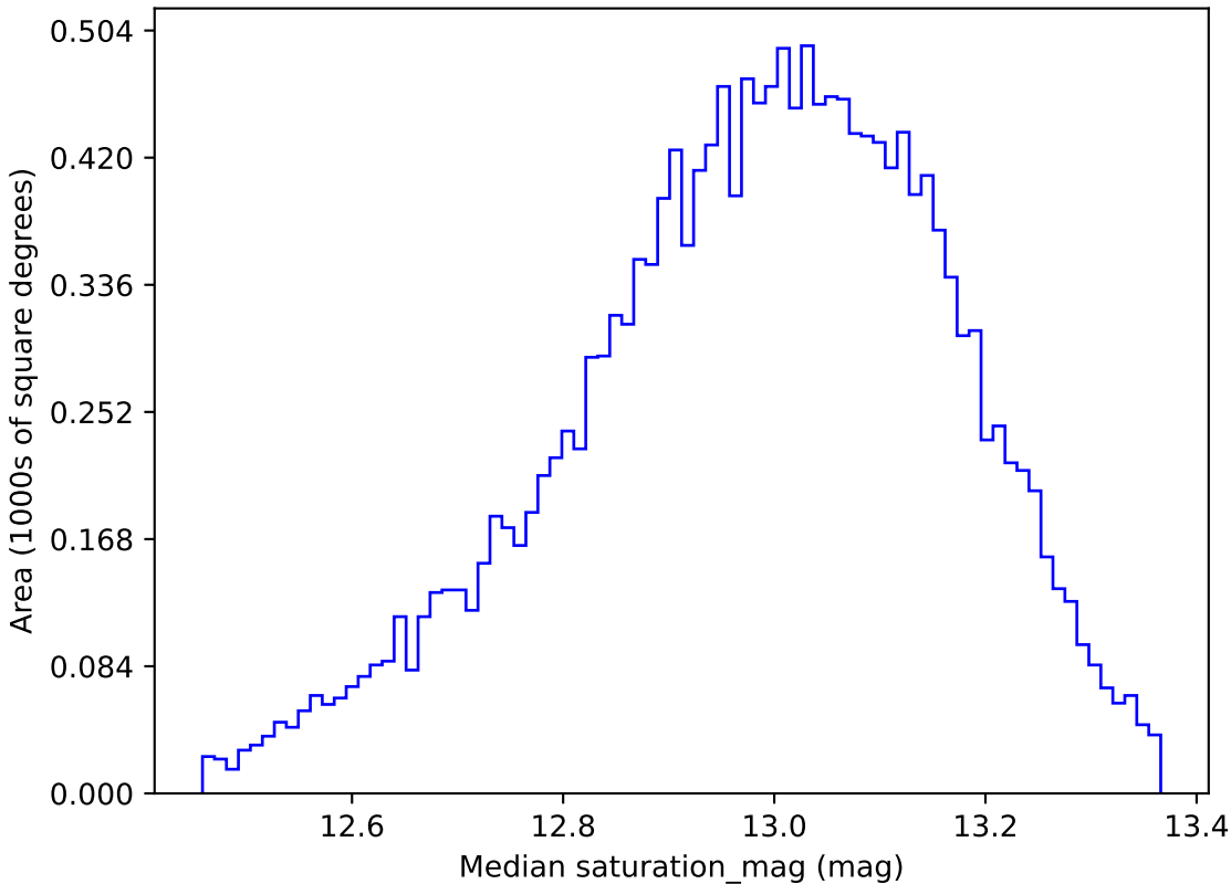
ddf_loaded_fl4_v3.4_10yrs WFD u band: Median saturation_mag
