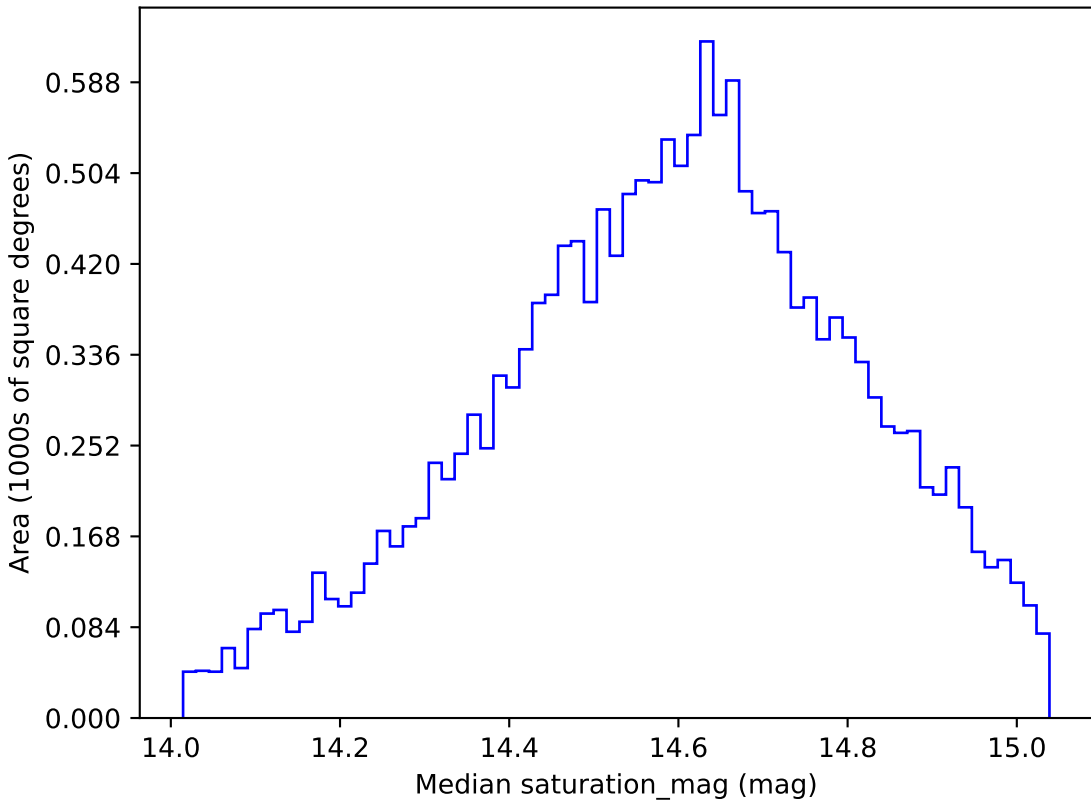
ddf_loaded_fl4_v3.4_10yrs WFD g band: Median saturation_mag
